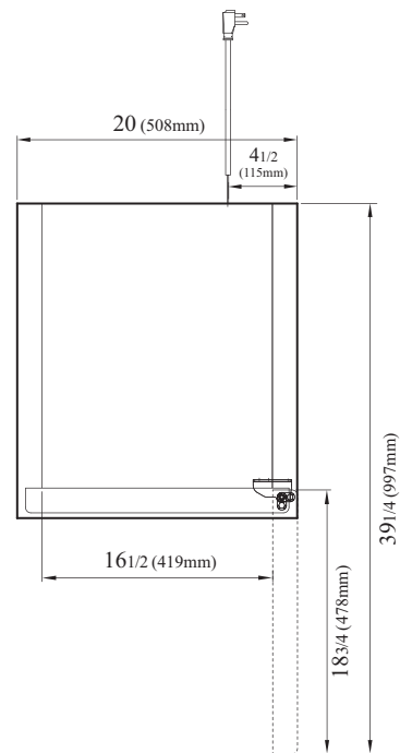
TOP VIEW
