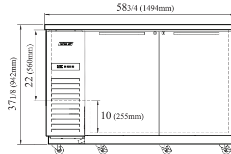
TBB-2SBD-N6 FRONT VIEW
