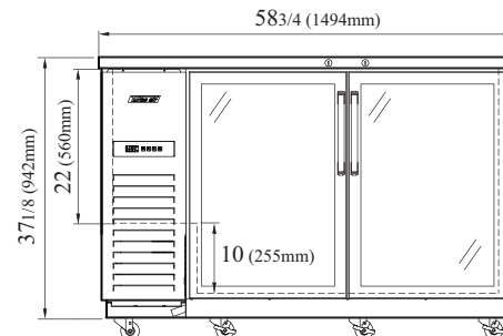
TBB-2SGD-N FRONT VIEW
