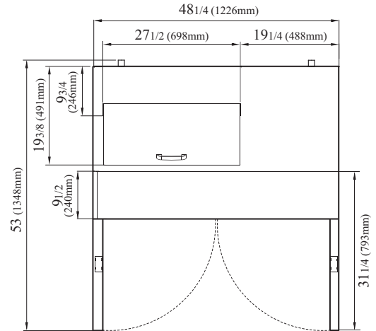
TST-48SD-08S-N TOP VIEW
