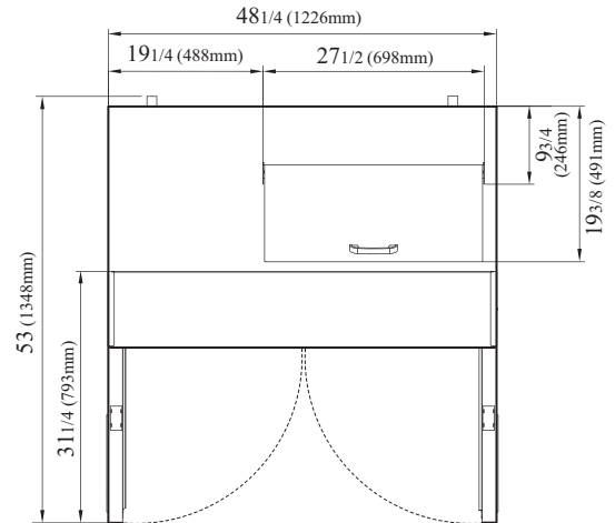
TST-48SD-08S-N-LW TOP VIEW
