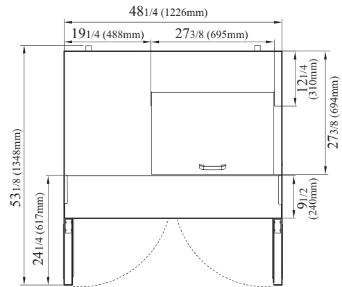
TST-48SD-12M-N-LW TOP VIEW
