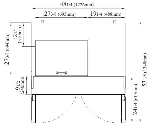
TST-48SD-12M-N TOP VIEW
