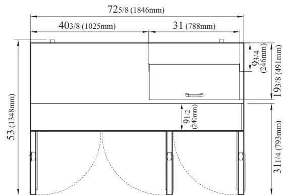
TST-72SD-08S-N-LW TOP VIEW
