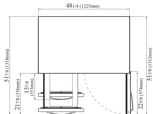
PUR-48-D2R-FB-N TOP VIEW
