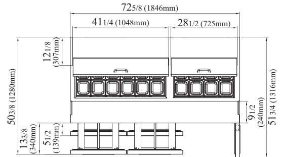
TST-72SD-30-D4R-FB-N TOP VIEW
