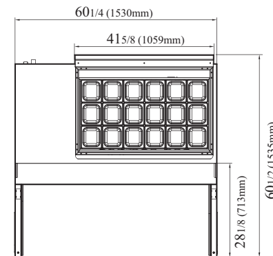
TST-60SD-18M-N-GL-LW TOP VIEW
