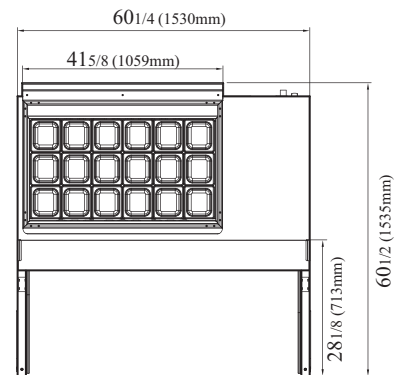
TST-60SD-18M-N-GL TOP VIEW
